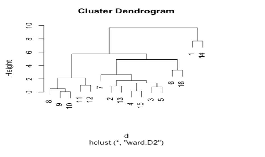
Figure B14: Clustering Daily Mean Series: Wavelet features
