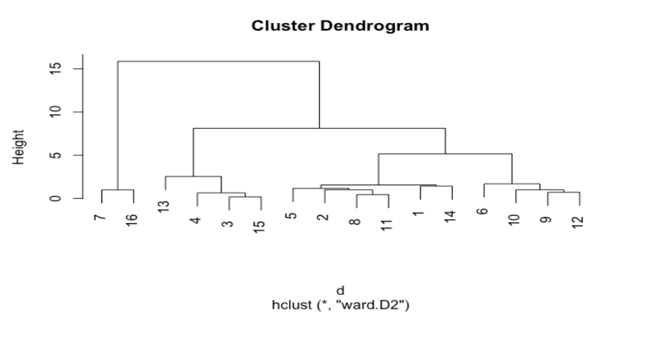
Figure B3: Clustering ITS: Space-time Coefficients
