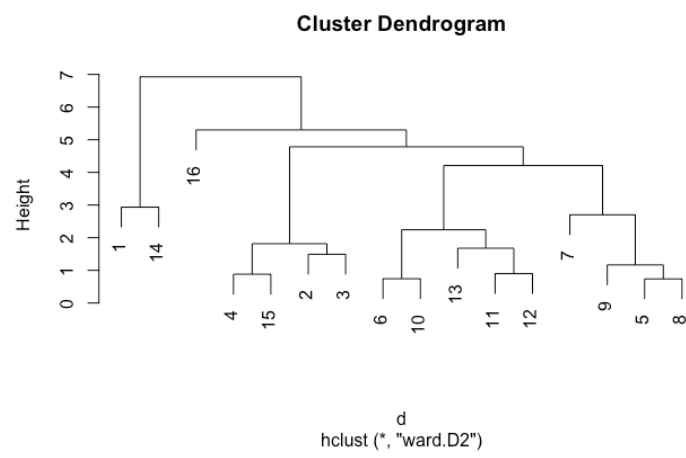
Figure B13: Clustering Daily Mean Series: Time Domain features
