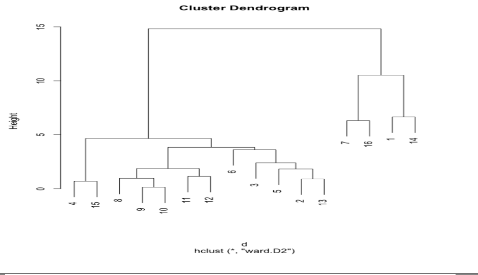
Figure B2: Clustering ITS: Wavelet Variances
