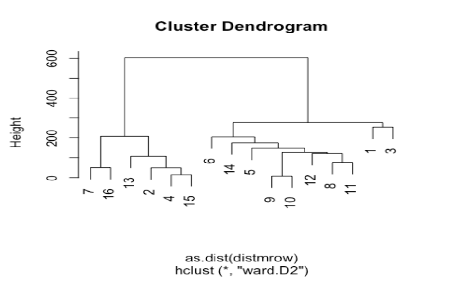
Figure B10: Clustering ITS: Correlation-based: Maximum absolute row sum
