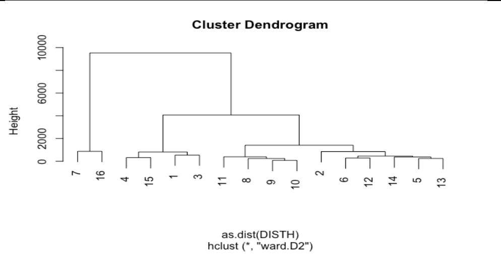
Figure B5: Clustering ITS: Point-to-Point: Hausdorff
