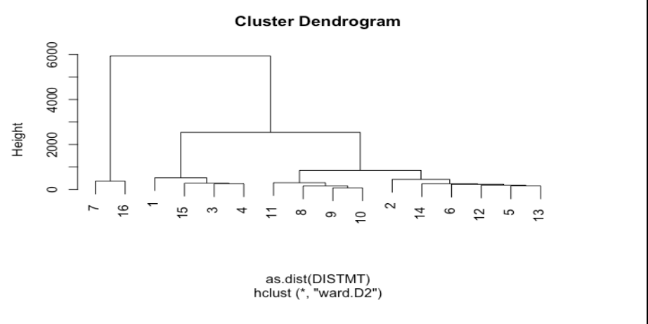
Figure B7: Clustering ITS Point-to-Point: Mallows Triangular
