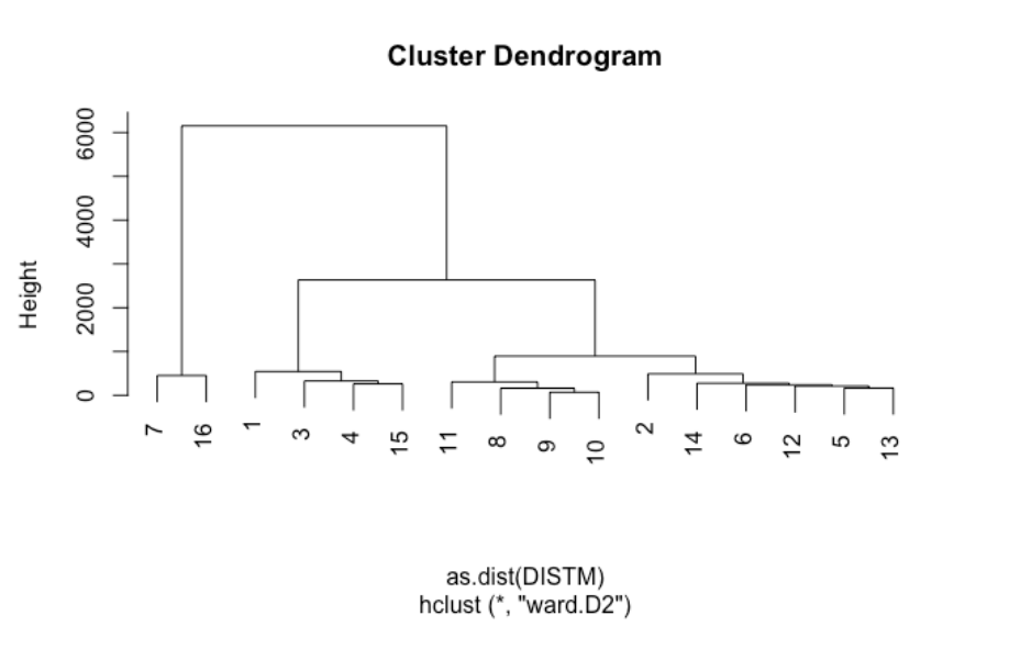
Figure B6: Clustering ITS: Point-to-Point: Mallows Uniform
