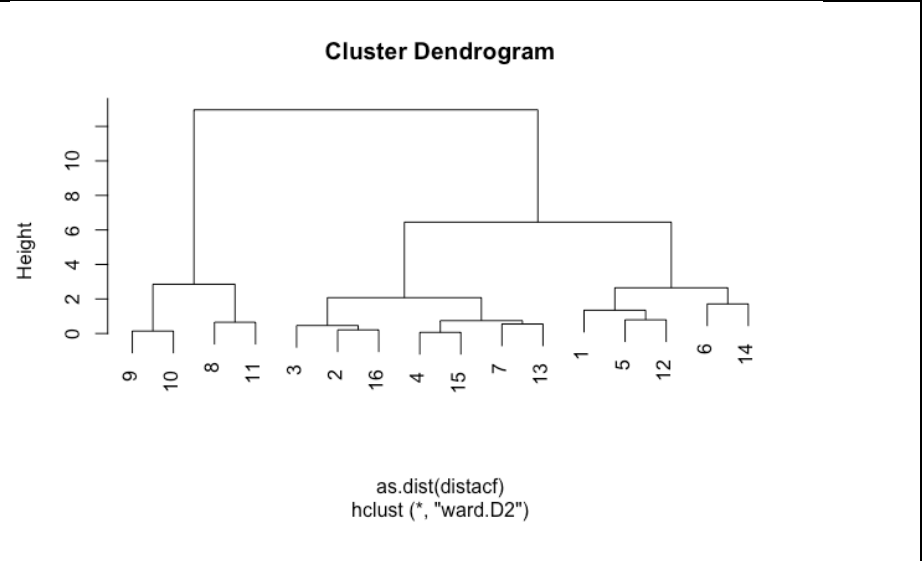
Figure B12: Clustering ITS: Interval ACF
