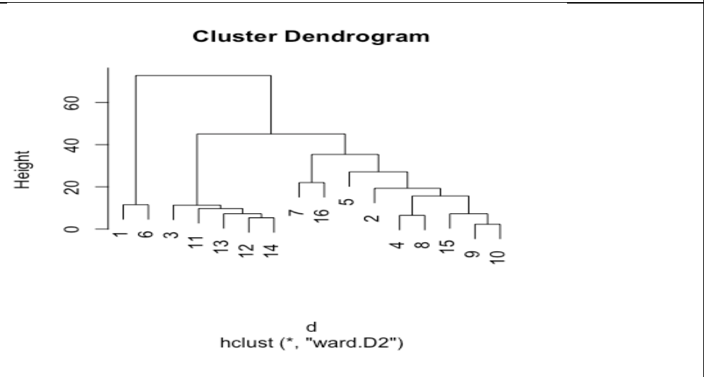
Figure B16: Clustering Daily Mean: Autocorrelation-based
