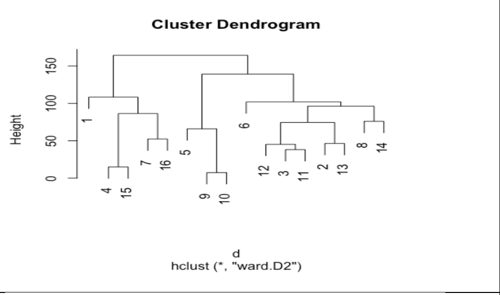
Figure B15: Clustering Daily Mean Series: Observations-based
