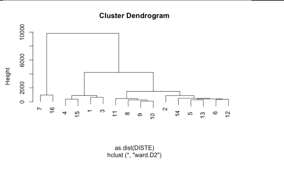
Figure B4: Clustering ITS: Point-to-Point: Euclidean
