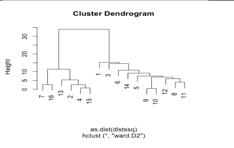
Figure B8: Clustering ITS: Correlation-based: Frobenius
