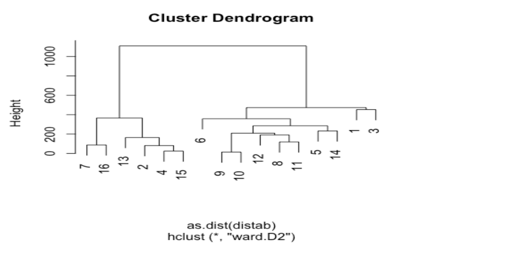
Figure B9: Clustering ITS: Correlation-based: Absolute value difference
