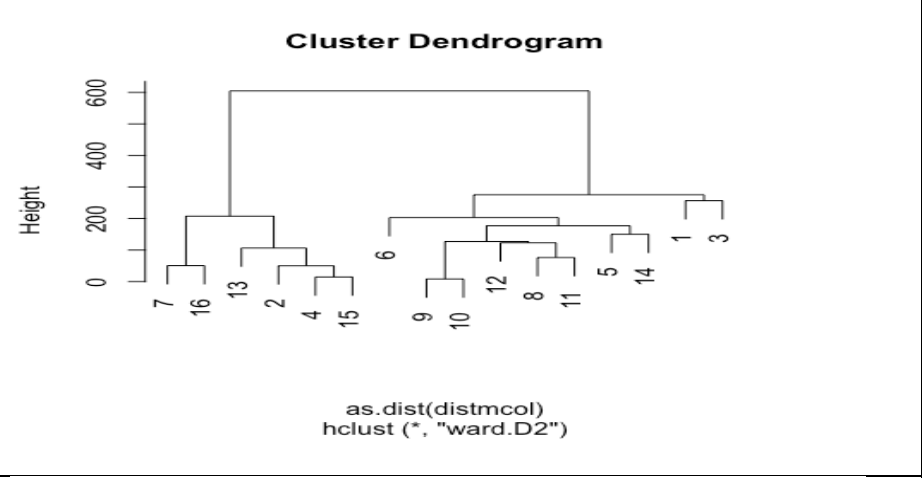
Figure B11: Clustering ITS: Correlation-based: Maximum absolute column sum
