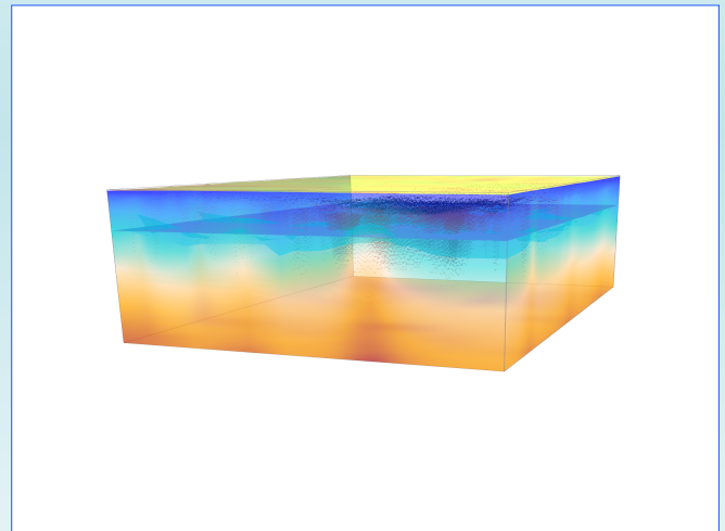
Figure 1: 3D Underworld model of Cooper Basin geothermal properties, visualised using gLucifer (to view and rotate interactively in 3D, open in Acrobat Reader v. 8.0 or higher).
