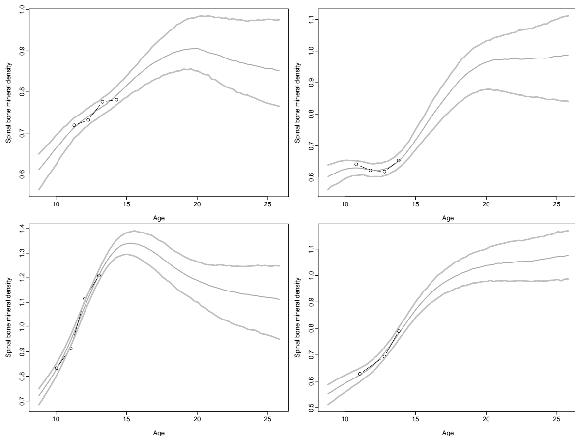
Figure 3: Interpolation and extrapolation of the spinal bone mineral density (g/sm 2 ) for cases 1, 3, 4 and 190.
