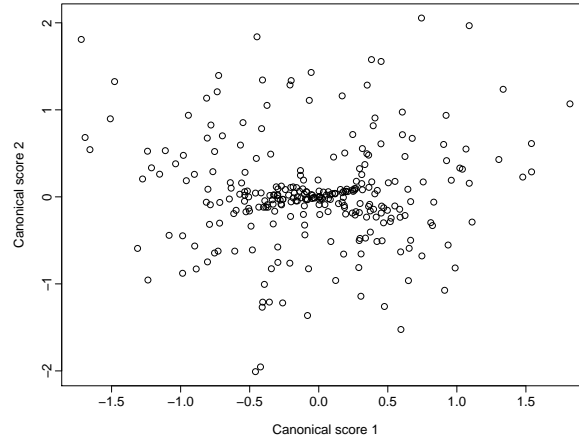
Figure 6: Scatter plot of the first two canonical scores of the spinal bone mineral density dataset.
