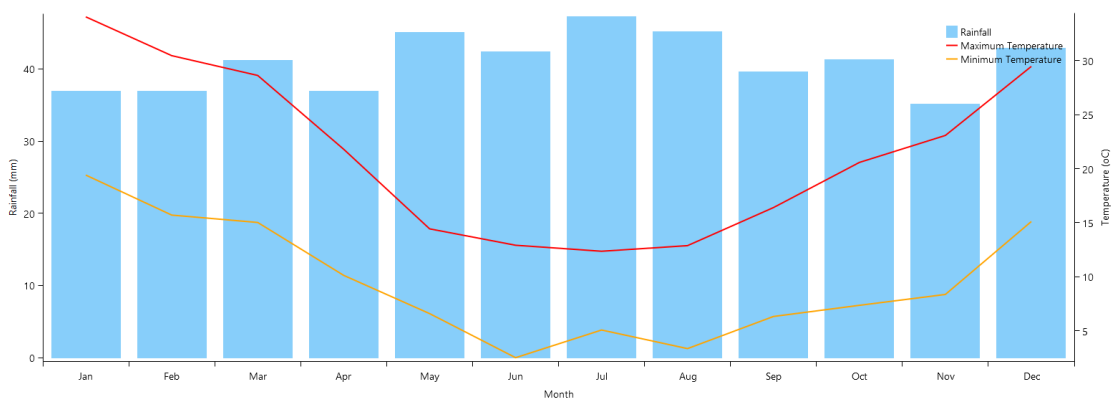
Wagga Wagga Average Climate Data 1960–2015 With Lower-Bound Predicted Climate Change
