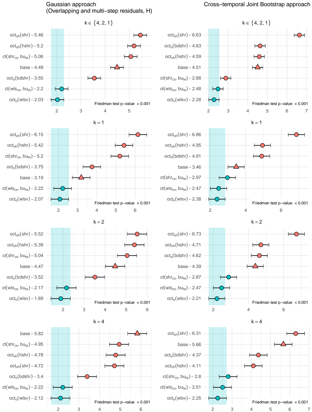
Figure 8: MCB Nemenyi test for the Australian QNA dataset using CRPS at different temporal aggregation levels for the Gaussian (using overlapping and multi-step residuals, H) and the non-parametric bootstrap approaches. In each panel, the Friedman test p-value is reported in the lower right corner. The mean rank of each approach is shown to the right of its name. Statistical differences in performance are indicated if the intervals of two forecast reconciliation procedures do not overlap. Thus, approaches that do not overlap with the blue interval are considered significantly worse than the best, and vice-versa.
