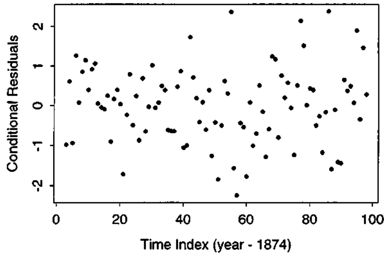
Figure 11: Plot of standardised conditional residuals for the Lake Huron data.
