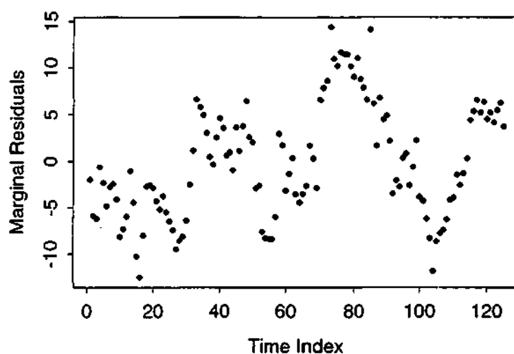
Figure 1: An example of a plot of marginal residuals where the error model is AR(1) . The pattern dominating the plot is due to autocorrelation.
